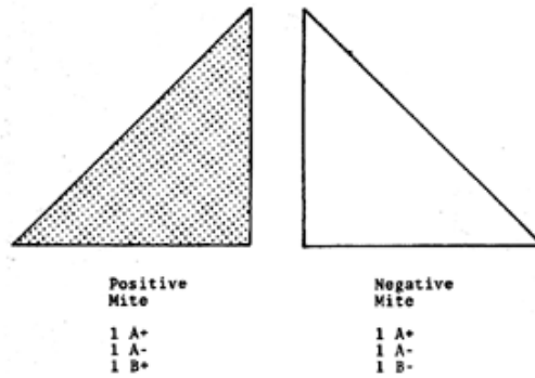
Fig. 954.00A A and B Quanta Module Orientations.
