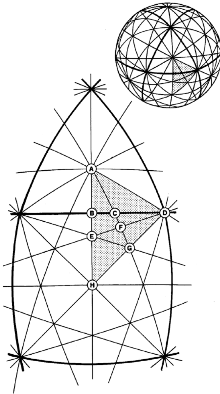
Fig. 453.01 Great Circles of Vector Equilibrium Define Lowest Common Multiple Triangle: 1/48th of a Sphere: The shaded triangle is 1/48th of the entire sphere and is the lowest common denominator (in 24 rights and 24 lefts) of the total spherical surface. The 48 LCD triangles defined by the 25 great circles of the vector equilibrium are grouped together in whole increments to define exactly the spherical surface areas, edges, and vertexes of the spherical tetrahedron, spherical cube, spherical octahedron, and spherical rhombic dodecahedron. The heavy lines are the edges of the four great circles of the vector equilibrium. Included here is the spherical trigonometry data for this lowest-common-denominator triangle of 25-great-circle hierarchy of the vector equilibrium.
