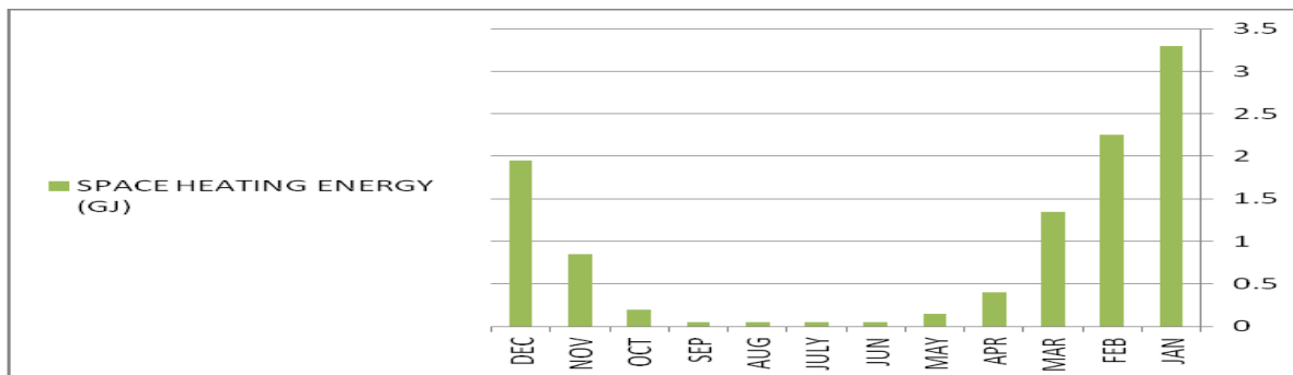
Figure 19: Monthly space heating energy consumed by the active energy system.
