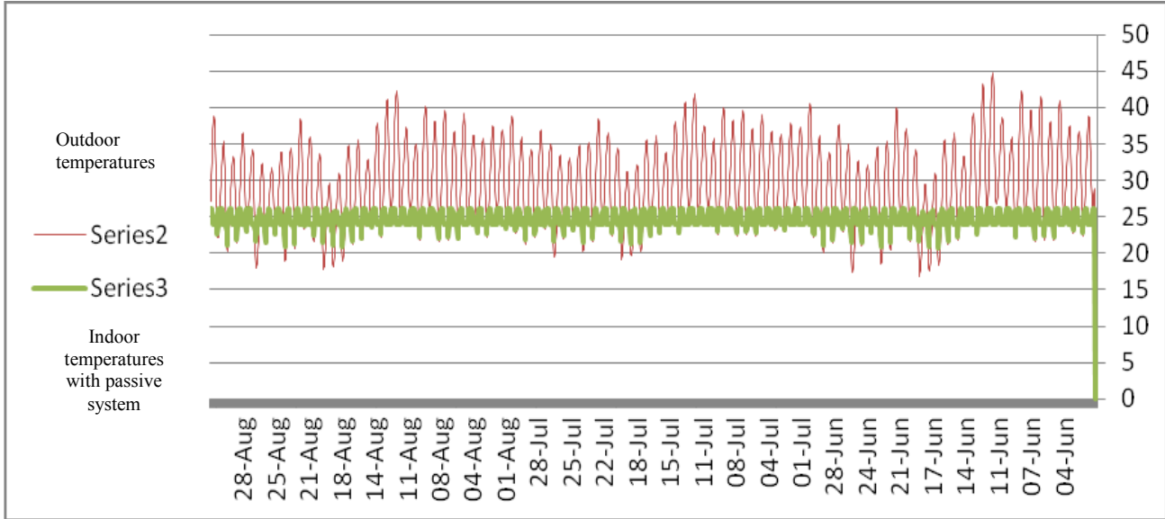
Figure 16: The hourly difference between the outdoor temperatures, and the indoor temperature for reception area with use of passive system (without HVAC) in the hot season (June, July & august).
