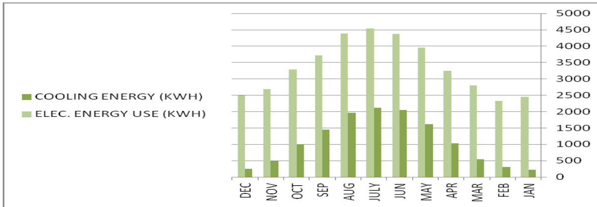
Figure 18: Monthly electric energy and Monthly Cooling energy consumed by the active energy system.
