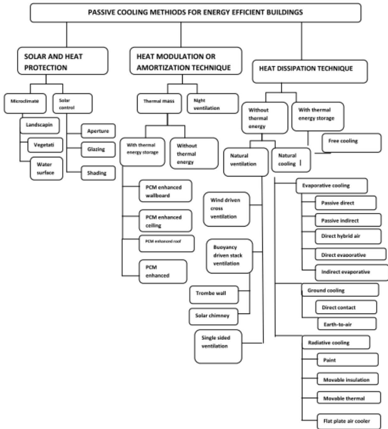
Figure 1: Classification of passive cooling methods in energy efficient buildings.
