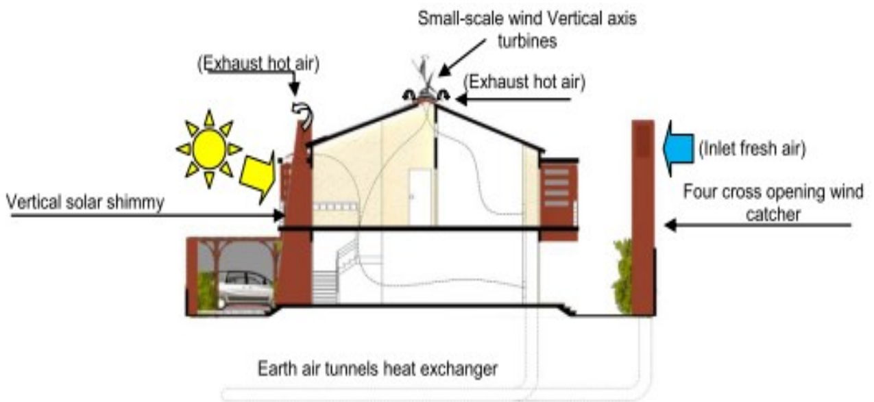
Figure 7: Suggested prototype smart house cross section.
