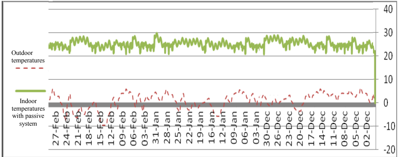
Figure 14: The hourly difference between the outdoor temperatures, and the indoor temperature for reception area with use of passive system (without HVAC) in the cold season (December, January & February)
